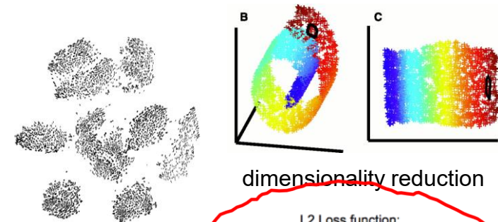
clustering
