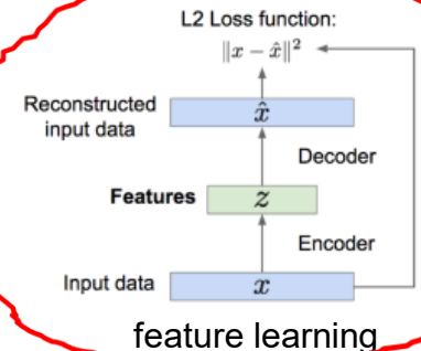
dimensionality reduction
